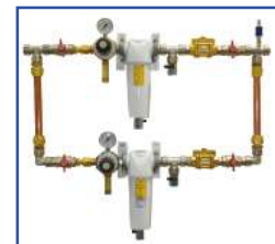
Duplex parallel pressure release line
